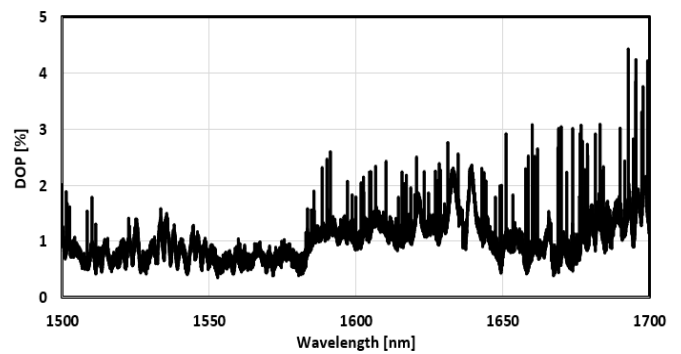
FIG. 8: DEGREE OF POLARIZATION
