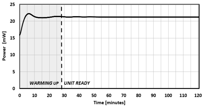
FIG. 9: WARM-UP TIME
