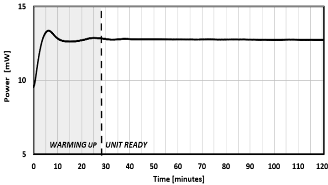
FIG. 7: WARM-UP TIME
