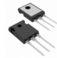
IRFP048PBF Vishay Siliconix MOSFET N-CH 60V 70A TO-247AC
